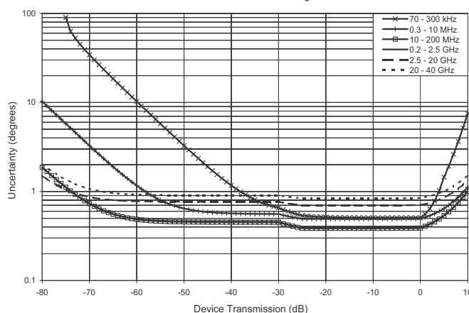
Transmission Phase Uncertainty MS4644B with SOLT Calibration using 3652A Cal Kit
