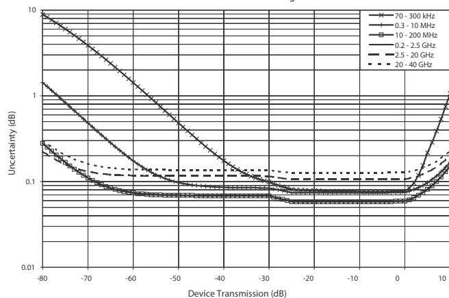
Transmission Magnitude Uncertainty MS4644B with SOLT Calibration using 3652A Cal Kit
