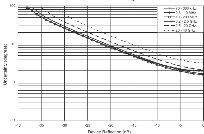
Reflection Phase Uncertainty MS4644B with SOLT Calibration using 3652A Cal Kit
