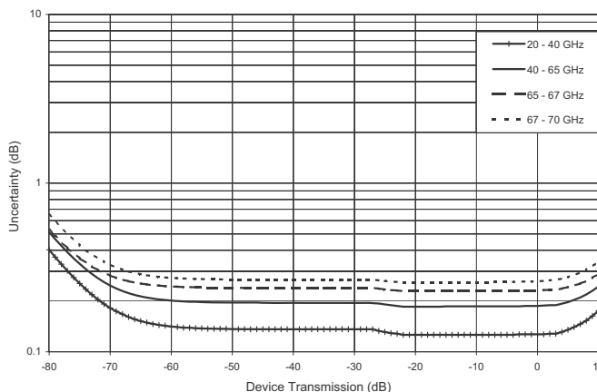
Transmission Magnitude Uncertainty (2 of 2) MS4647B with SOLT-SL Calibration using 3654D-1 Cal Kit
