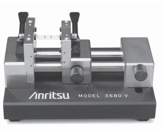
3680 Series Universal Test Fixture (UTF)
