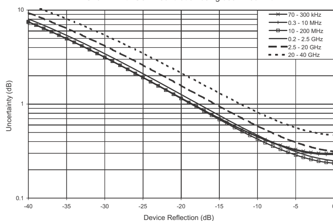
Reflection Magnitude Uncertainty MS4644B with SOLT Calibration using 3652A Cal Kit
