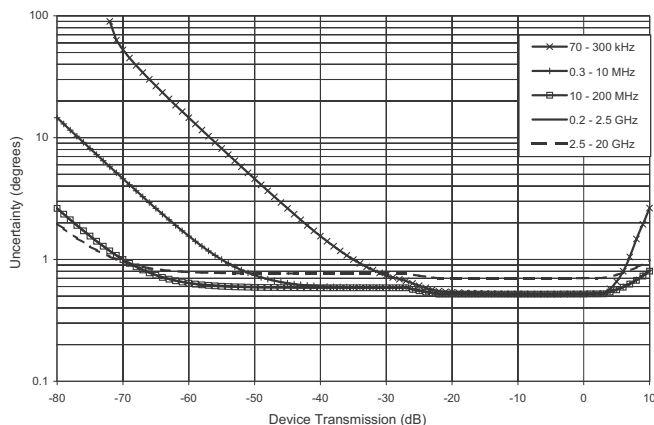
Transmission Phase Uncertainty (1 of 2) MS4647B with SOLT-SL Calibration using 3654D-1 Cal Kit
